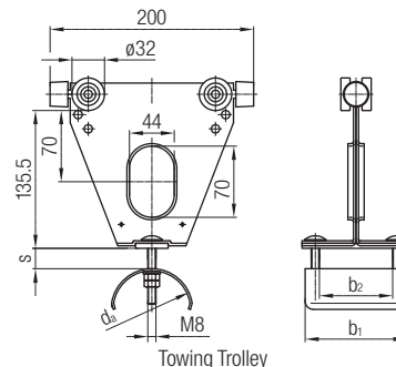
Towing Trolley
