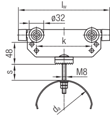
Cable Trolley
