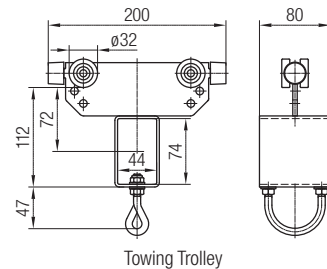
Towing Trolley
