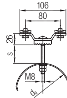
End Clamp
